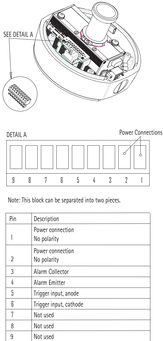
Figure 2 Power and Network Connections
